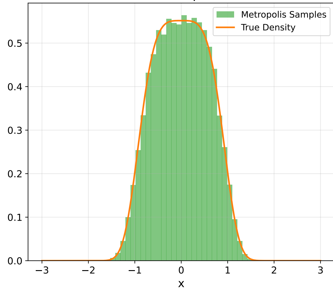
Normal(0, 0.75), Acceptance Rate=0.68
