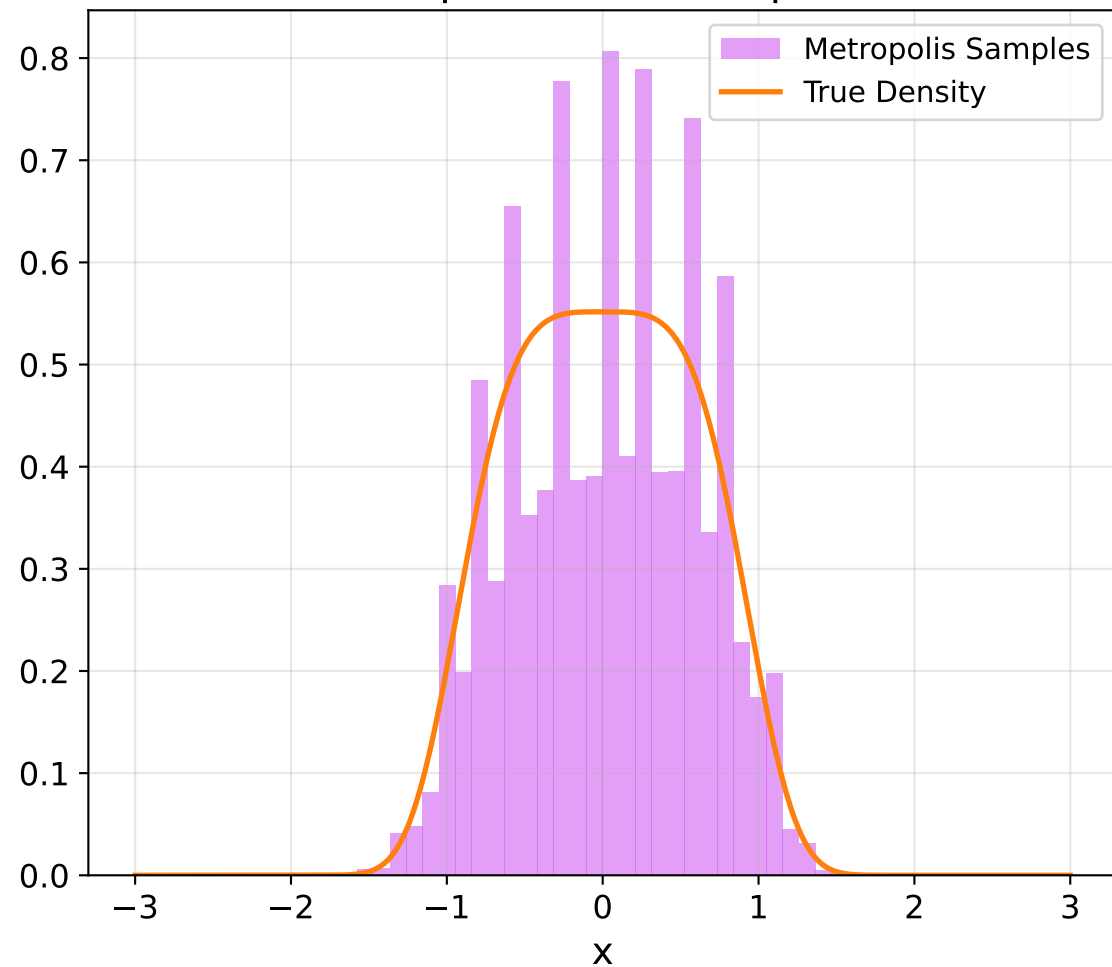
Random Walk (Step=0.075), Acceptance Rate=0.96
