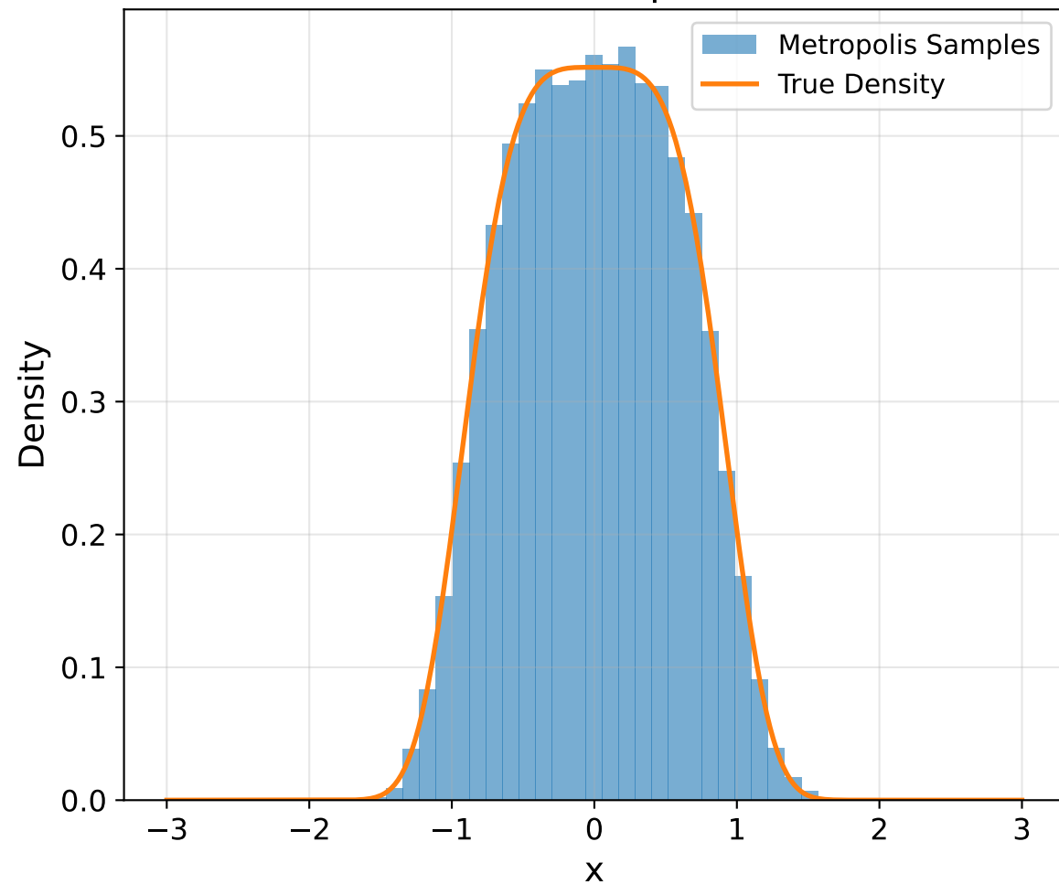
Uniform(-0.5, 0.5), Acceptance Rate=0.86
